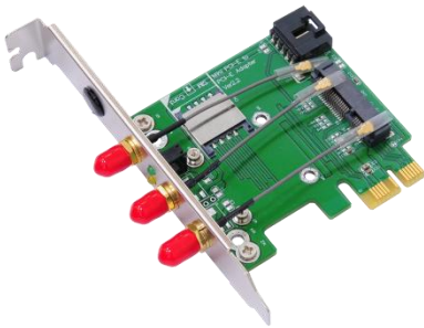
MP2W (Mini PCI-E / PCI-E Adapter ver 2.3) x1 with RF11005A x3
